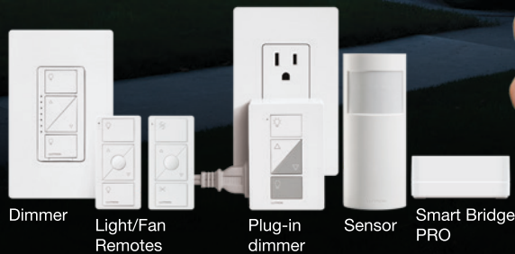
Lutron App
